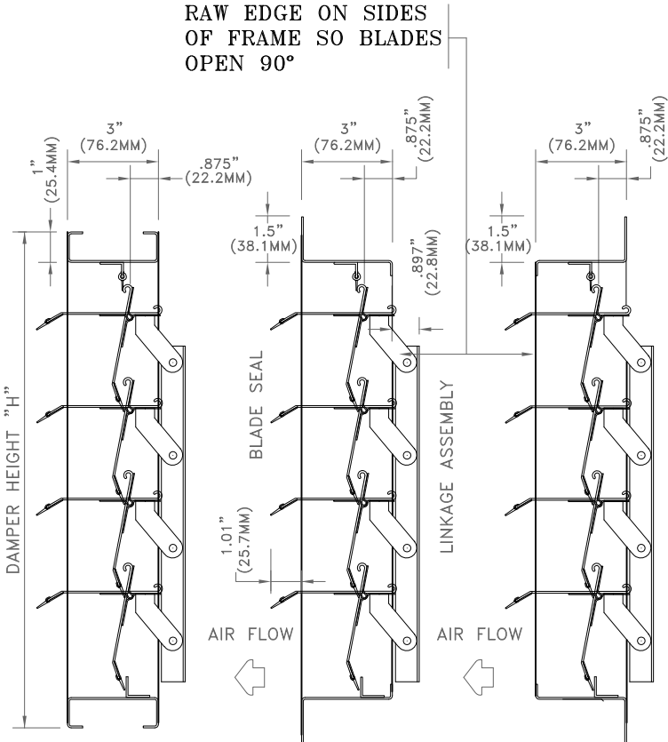
BDSS-3C3-LB SECTION STANDARD CHANNEL FRAME BDSS-3F3-LB SECTION OPTIONAL FLANGED FRAME BDSS-3RF-LB SECTION OPTIONAL REVERSE FLANGE FRAME
