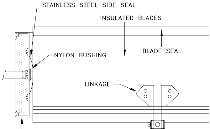
HORIZONTAL SECTION DETAIL (2:1 FROM DRAWING BELOW)
