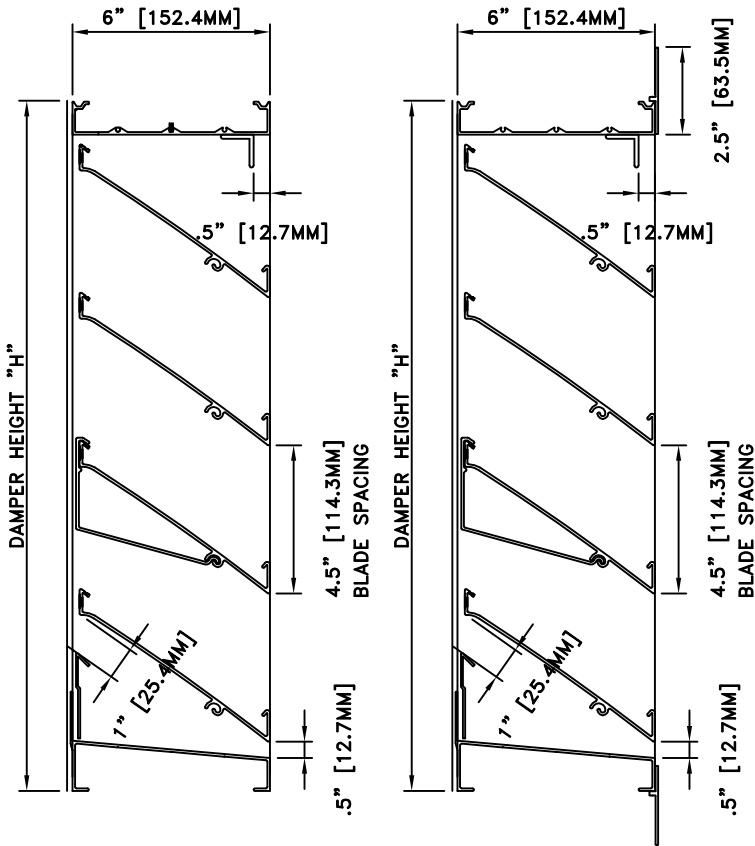
XT-635V VERTICAL SECTION
