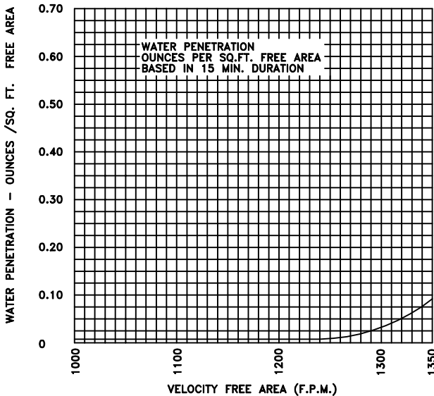
WATER PENETRATION GRAPH 1240 F.P.M. BEGINNING OF WATER PENETRATION (14.09 MPH WIND)
