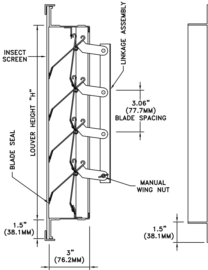
SECTION
