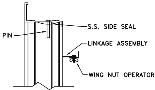
TOP VIEW (PARTIAL)
