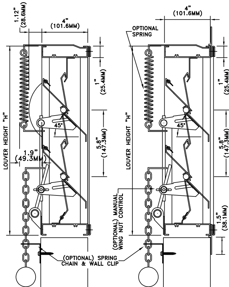
XC-445W-0 VERTICAL SECTION
