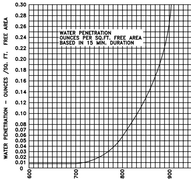
WATER PENETRATION GRAPH 700 F.P.M. BEGINNING OF WATER PENETRATION (7.95 MPH WIND)
