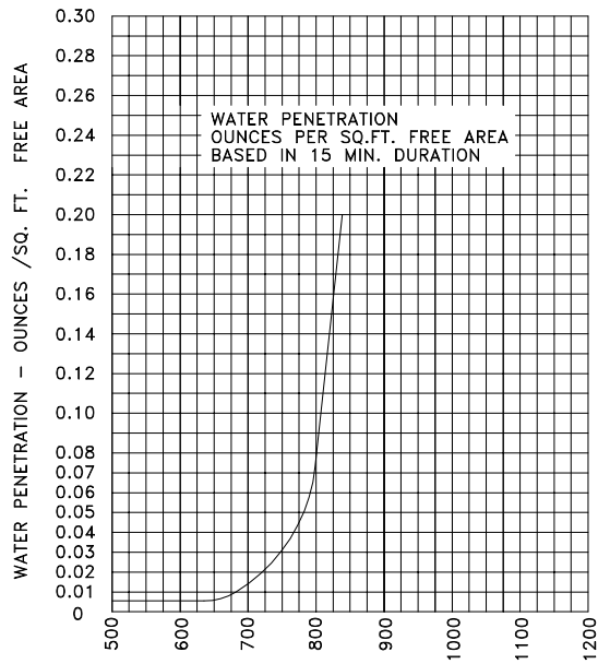
WATER PENETRATION GRAPH 650 F.P.M. BEGINNING OF WATER PENETRATION (7.4 MPH WIND)
