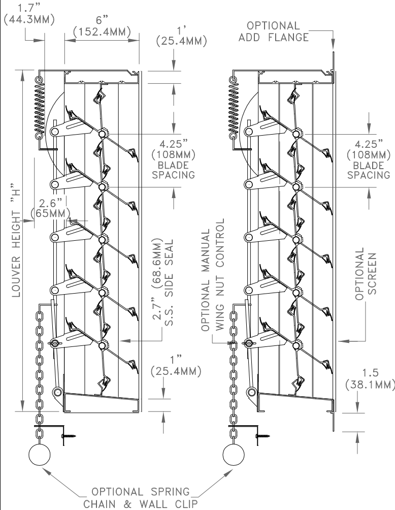
XC-635WV-0 VERTICAL SECTION
