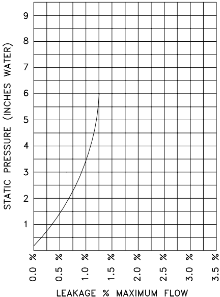
LEAKAGE GRAPH
