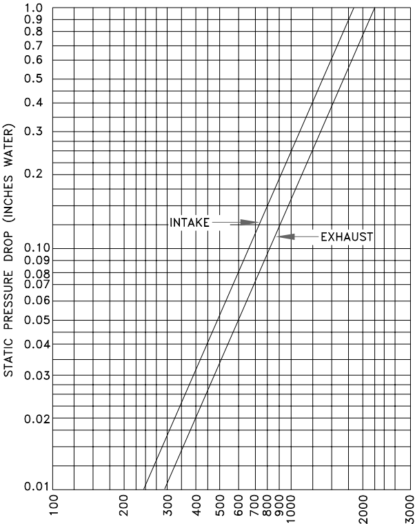
VELOCITY FREE AREA (F.P.M.) AIR PERFORMANCE GRAPH
