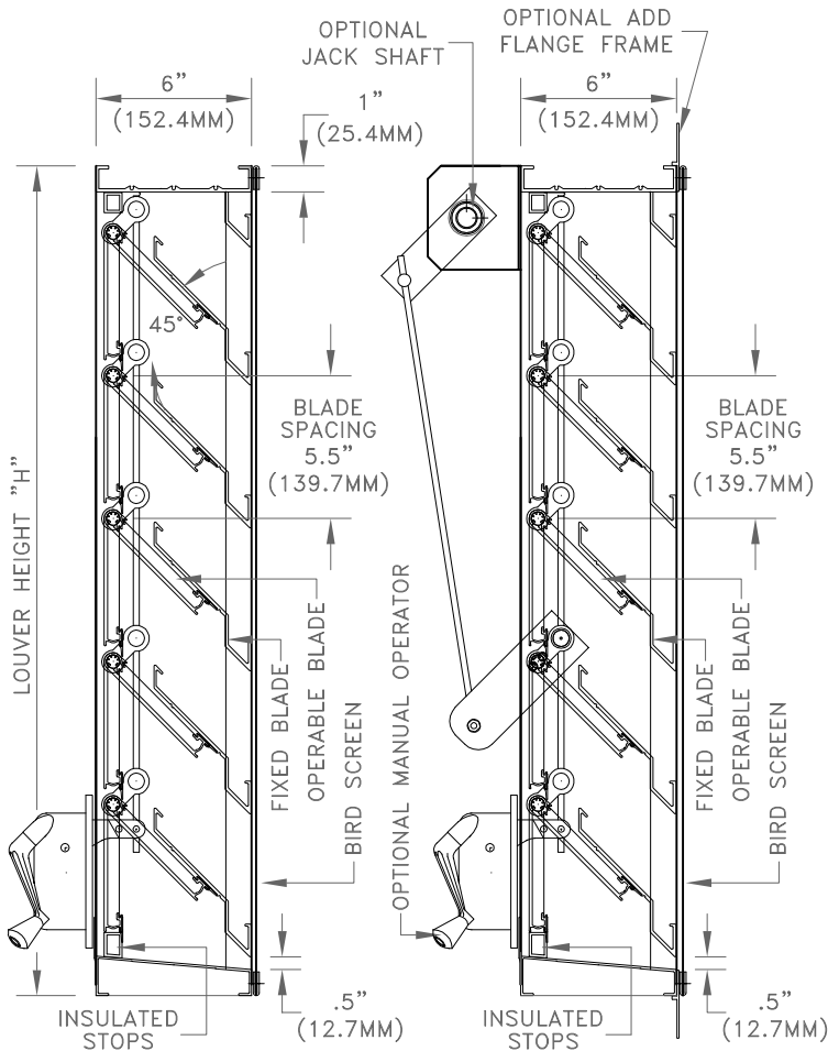
XT-640U-FO VERTICAL SECTION
