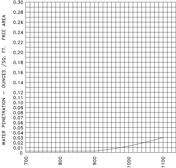
VELOCITY FREE AREA (F.P.M.) WATER PENETRATION GRAPH 900 F.P.M. BEGINNING OF WATER PENETRATION (10.23 MPH WIND)
