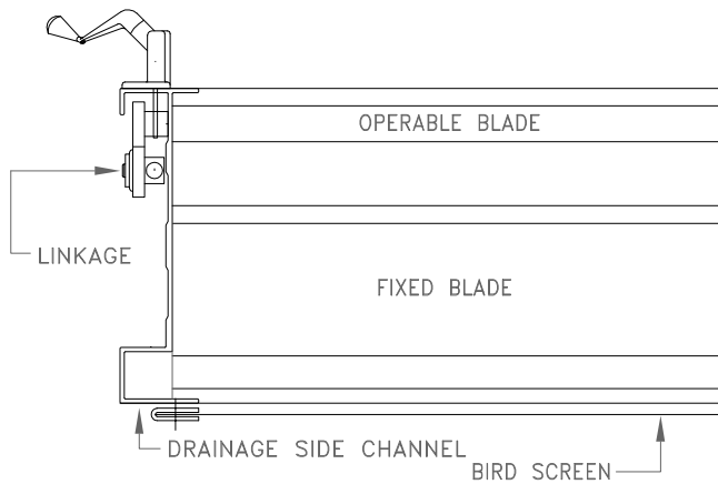
HORIZONTAL SECTION
