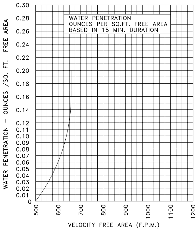
WATER PENETRATION GRAPH 500 F.P.M. BEGINNING OF WATER PENETRATION (5.68 MPH WIND)
