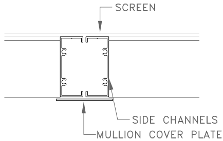
HORIZONTAL SECTION
