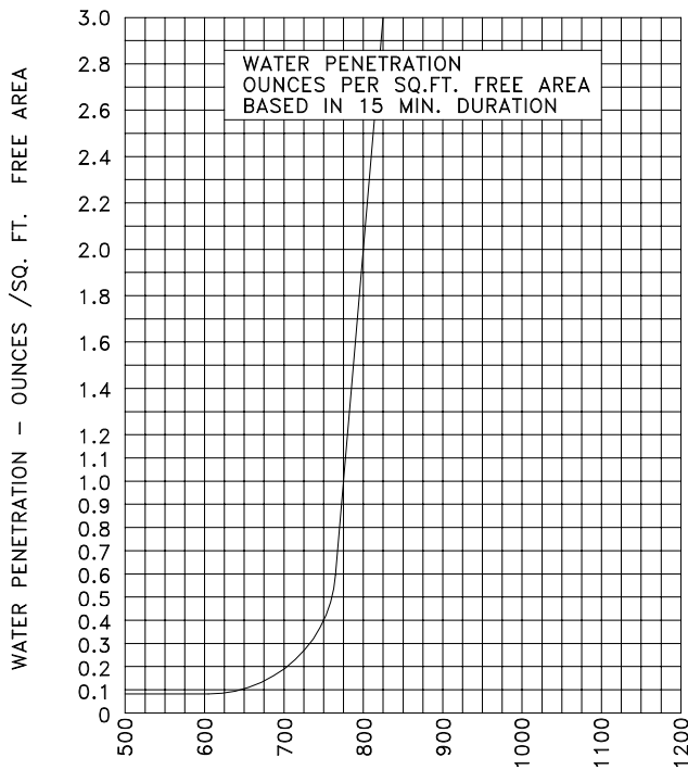
WATER PENETRATION GRAPH 605 F.P.M. BEGINNING OF WATER PENETRATION (6.88 MPH WIND)
