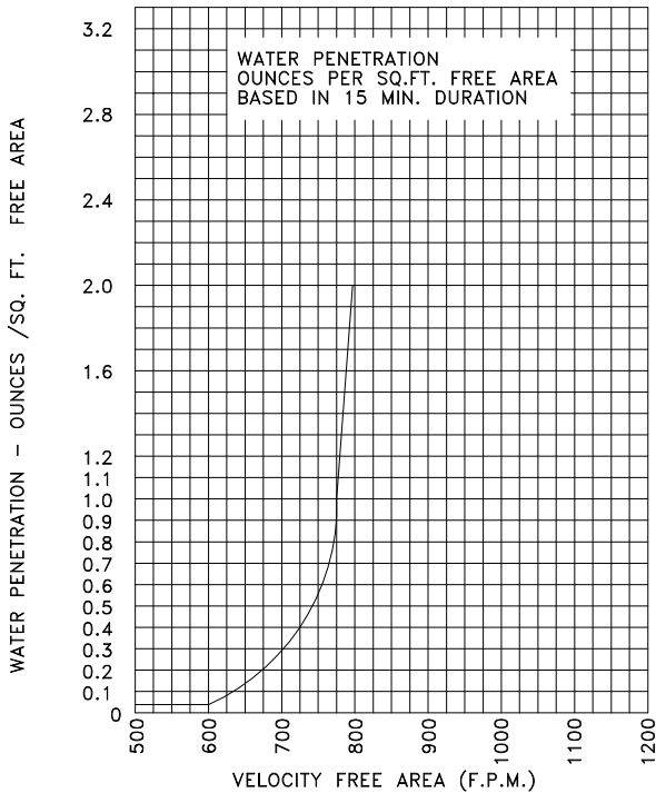
WATER PENETRATION GRAPH 605 F.P.M. BEGINNING OF WATER PENETRATION (6.88 MPH WIND)
