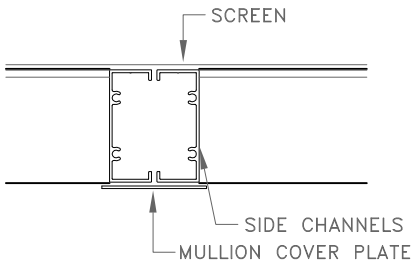
HORIZONTAL SECTION
