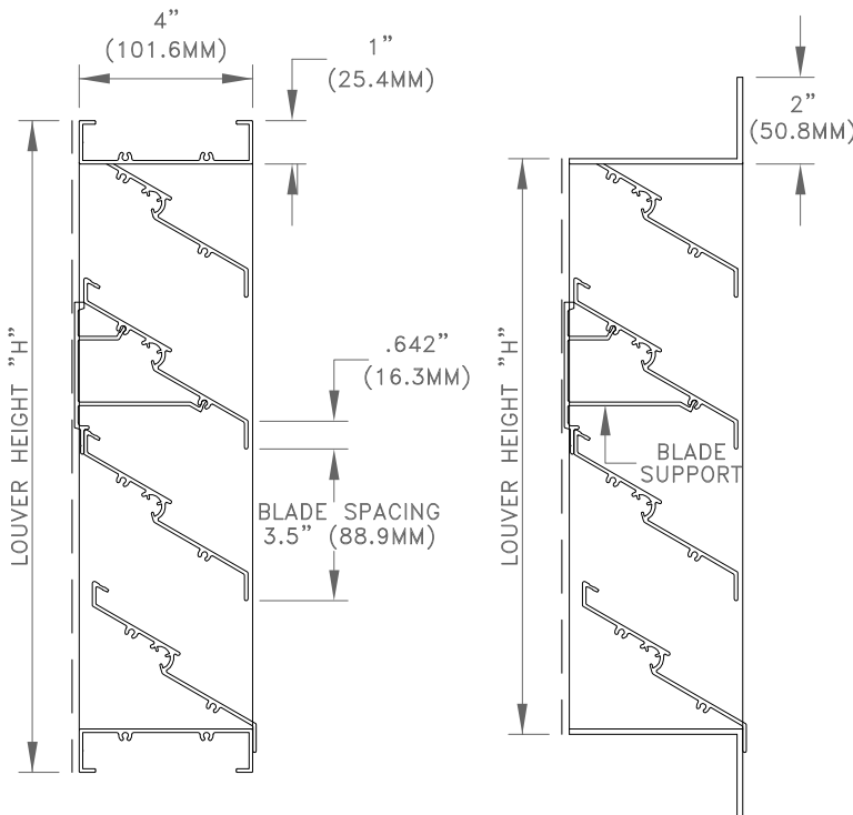
XC-430W XF-430W VERTICAL SECTION VERTICAL SECTION
