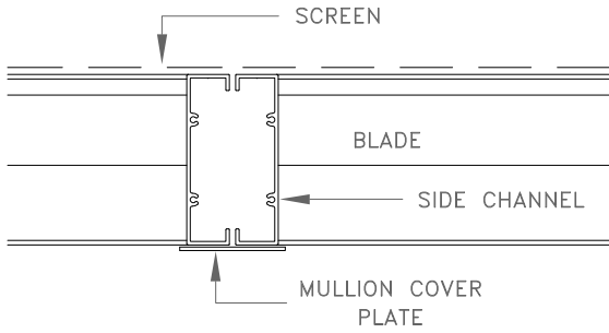
XF-430W HORIZONTAL SECTION
