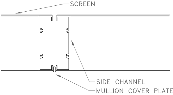
HORIZONTAL SECTION
