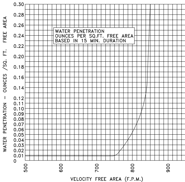
WATER PENETRATION GRAPH 744 F.P.M. BEGINNING OF WATER PENETRATION (8.45 MPH WIND)
