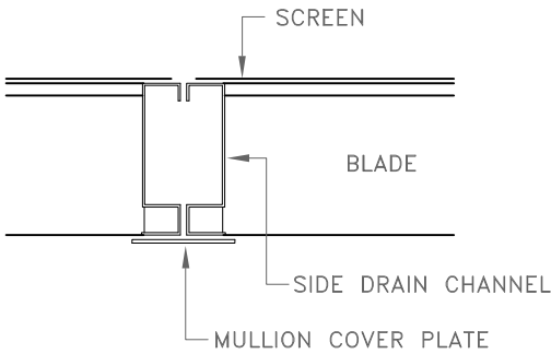
HORIZONTAL SECTION
