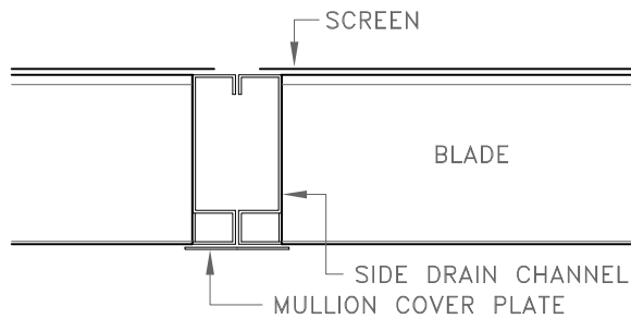
HORIZONTAL SECTION
