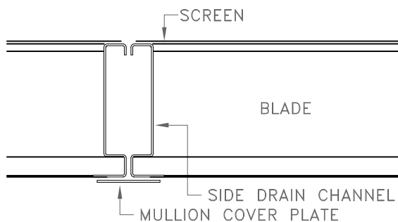
HORIZONTAL SECTION
