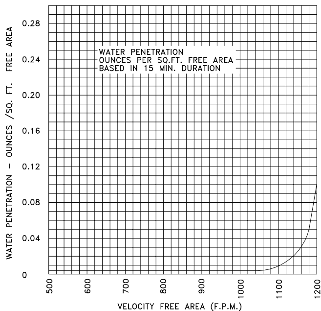
WATER PENETRATION GRAPH 1050 F.P.M. BEGINNING OF WATER PENETRATION (11.9 MPH WIND)
