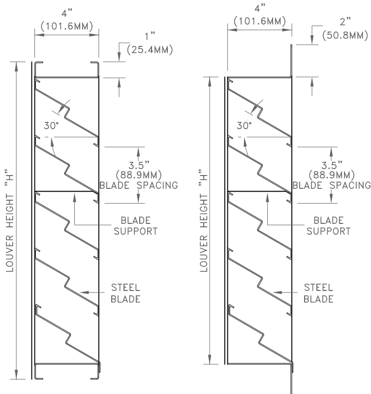
SC-430W SF-430W VERTICAL SECTION VERTICAL SECTION
