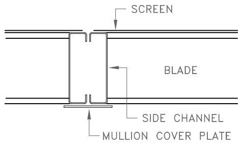
HORIZONTAL SECTION
