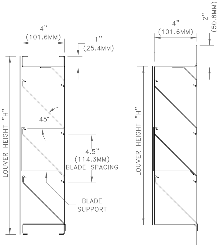
SC-445 VERTICAL SECTION
