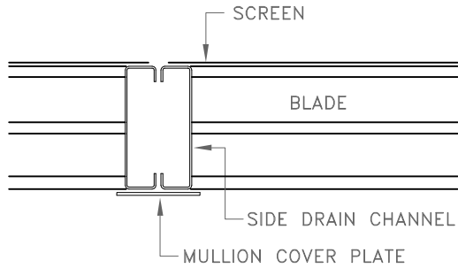
HORIZONTAL SECTION
