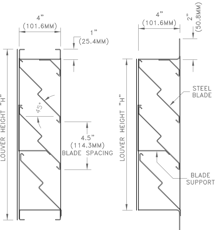
SC-445W VERTICAL SECTION
