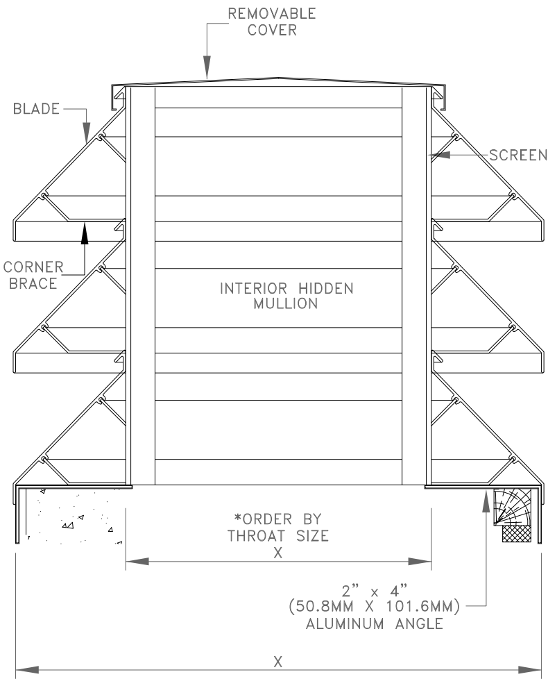
VERTICAL SECTION
