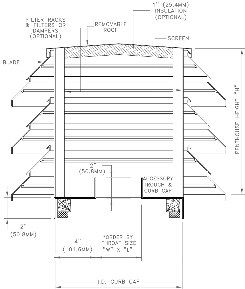
VERTICAL SECTION
